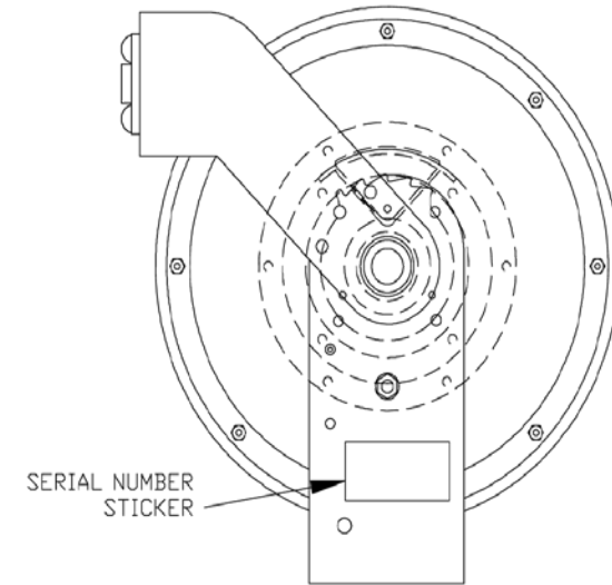
DRUM/RATCHET ORIENTATION DETAIL SEE NOTE 1
