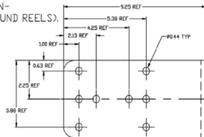
BASE MOUNTING
